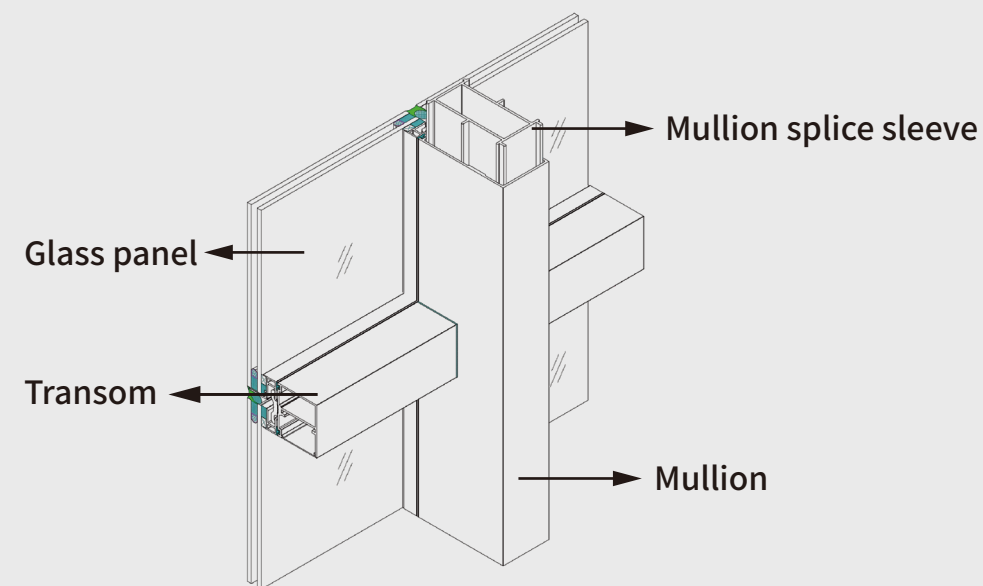
3D Detail of Hidden Frame Curtain Wall (Interior View)
